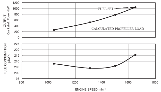
Medium Duty (1040kW / 1395HP / 1650rpm)
