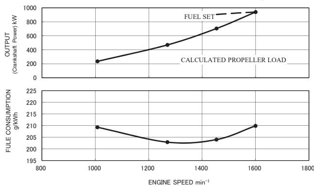
Heavy Duty (940kW / 1261HP / 1600rpm)
