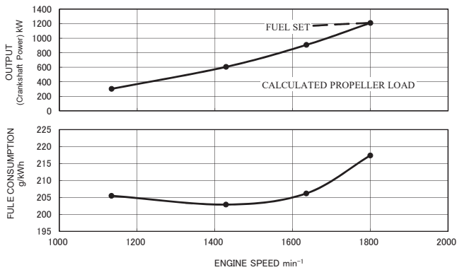
Light Duty (1210kW / 1623HP / 1800rpm)
